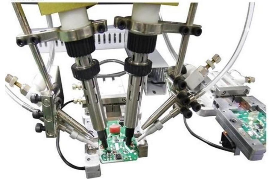
Welding head
